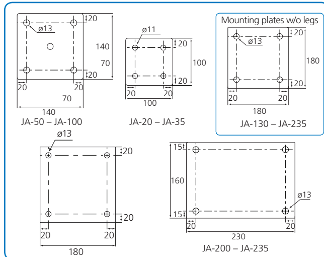
Base plate
